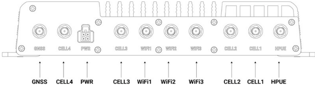
Figure 1 – MegaFi 2 SMA Connectors.
