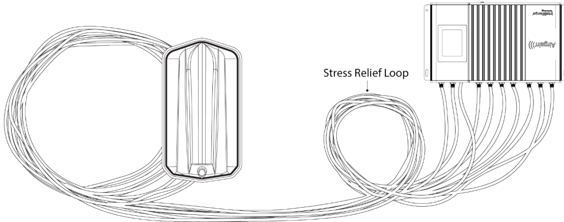
Figure 12 – Adding a stress relief loop.
