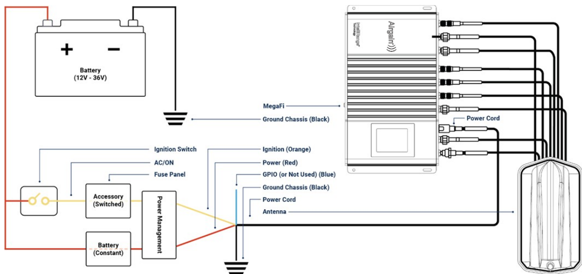
Figure 13 – Connecting DC power.
