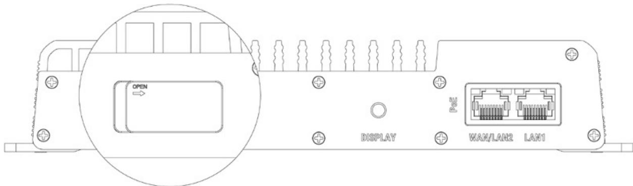
Figure 2 – Location of SIM slot, DISPLAY button, and networking ports.
