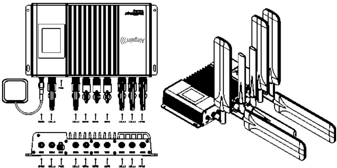
Figure 8 – Attaching the antennas
