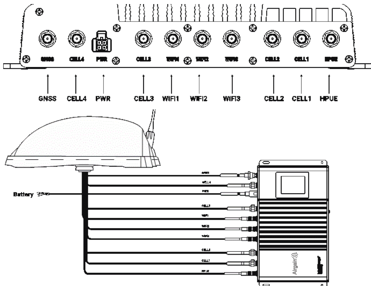
Figure 11 – Antenna port locations.
