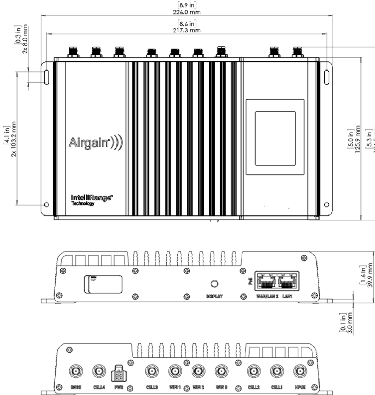
Figure 21 – MegaFi 2 dimensions.
